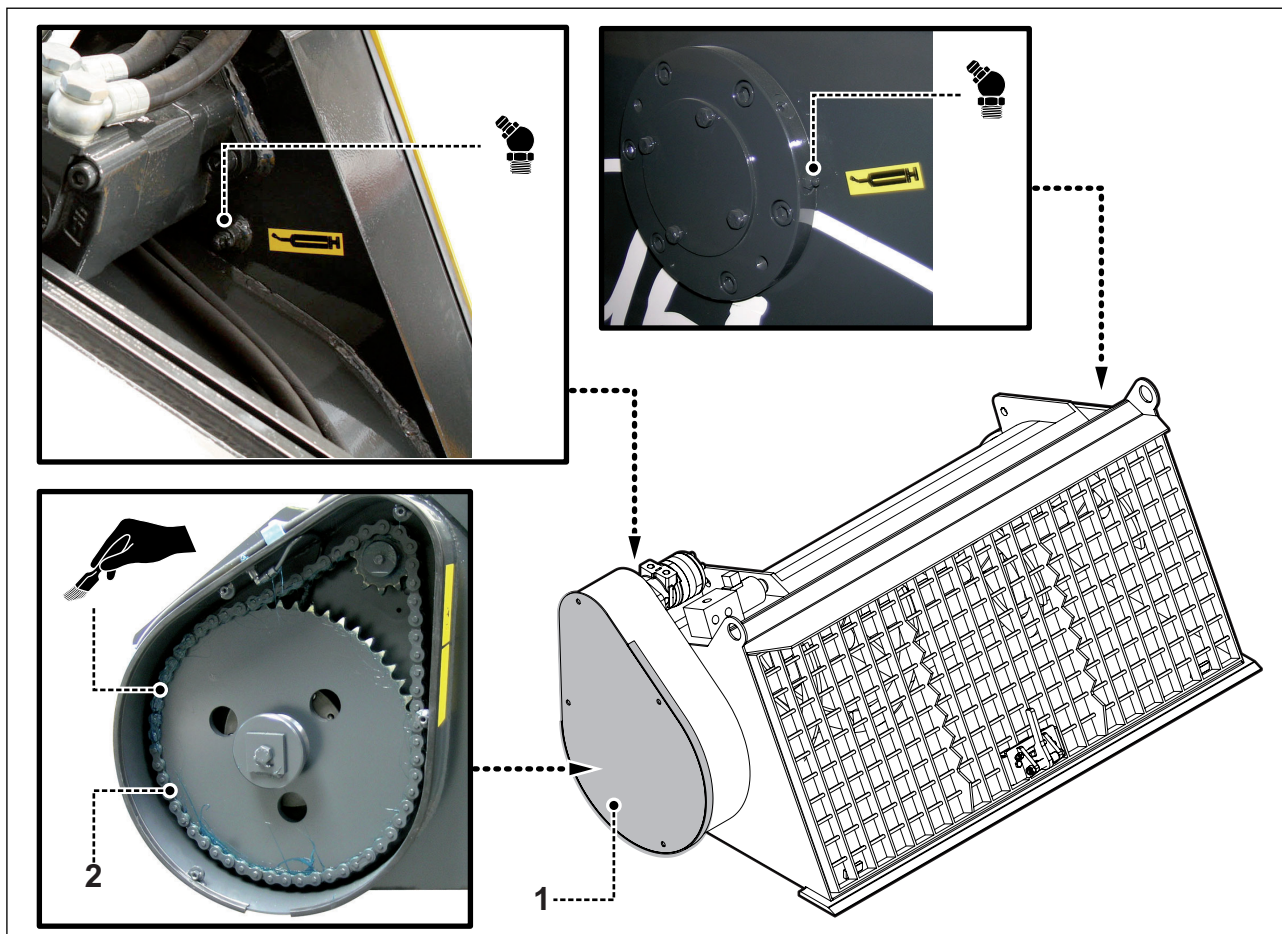
Greasing points diagram (Models 450-600-750-1000)
