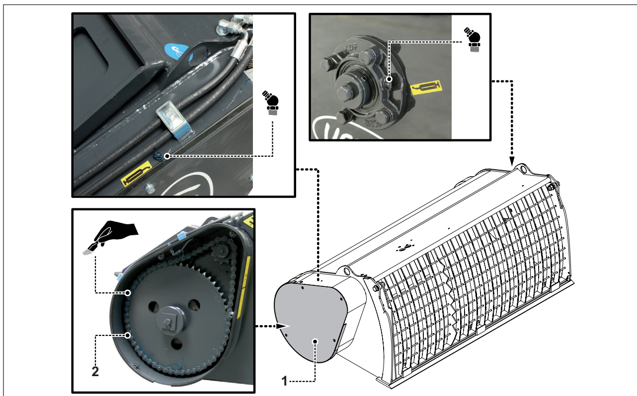
Greasing points diagram (Models 450-600-750-1000)
